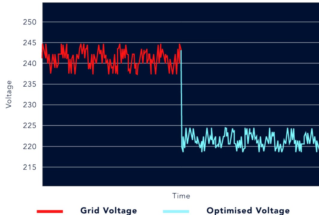
Grid supply voltage & optimised system voltage
